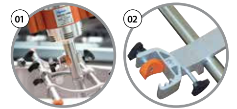
01 Top mounted support brackets 02 Side mounted support brackets
