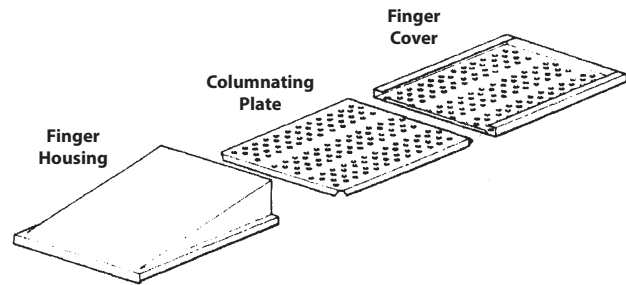
Top Finger Assembly
