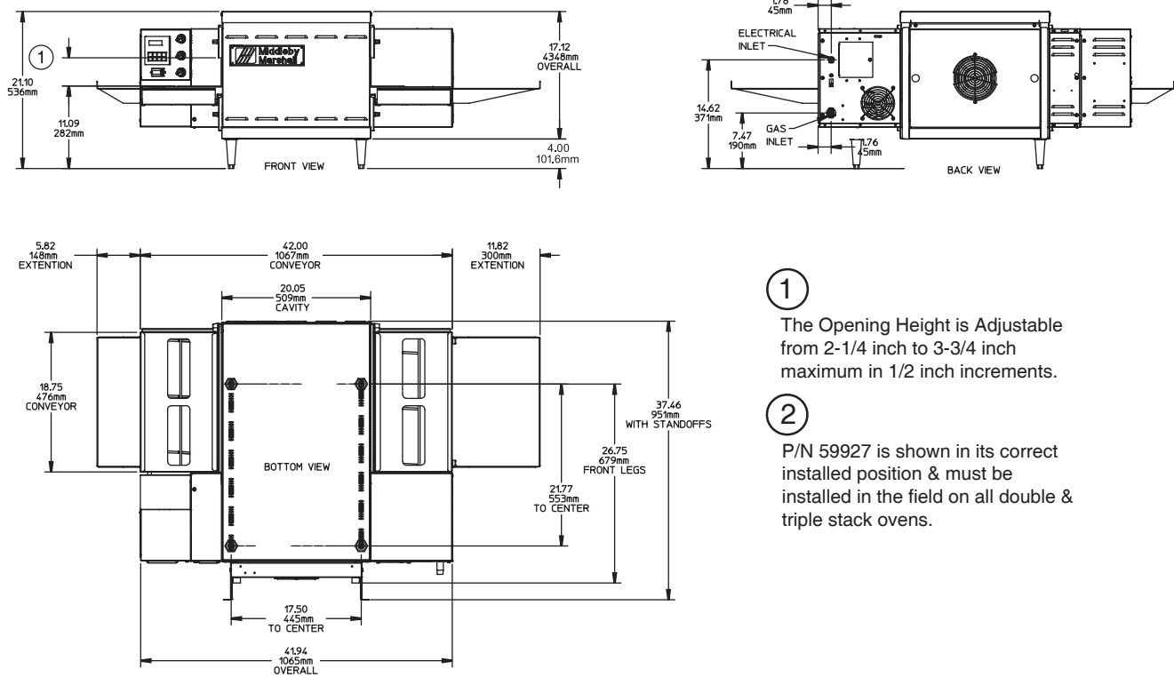
Figure 2-5. MODEL PS520 SINGLE OVEN DIMENSIONS
