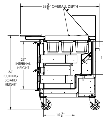
ELEVATION VIEW
