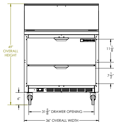
ELEVATION VIEW
