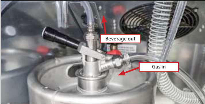
Fig. 11. Installed and connected taper.
