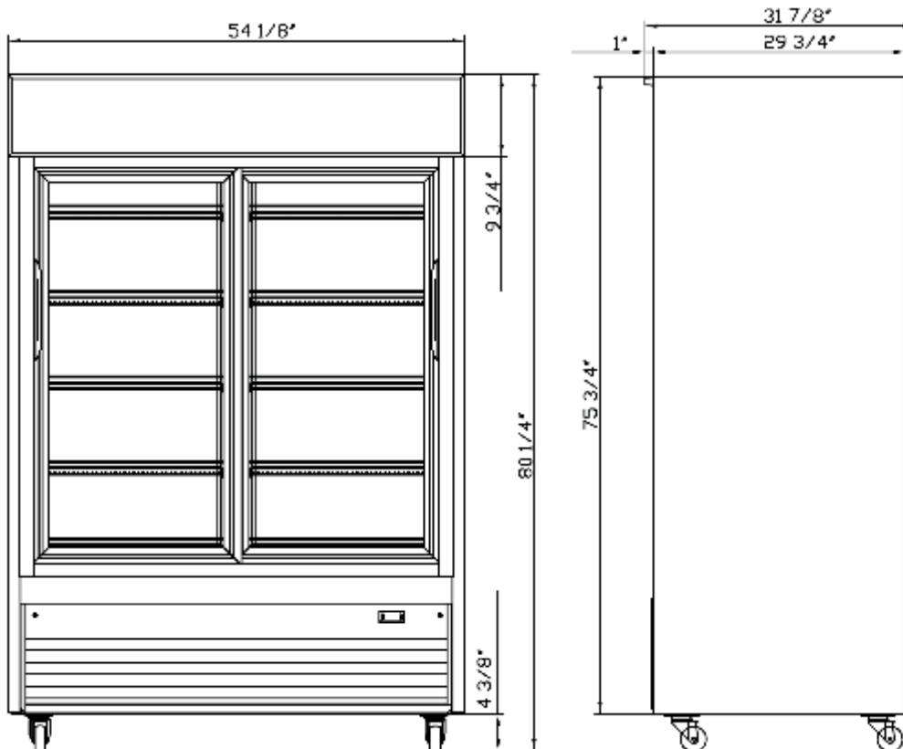
Front View
