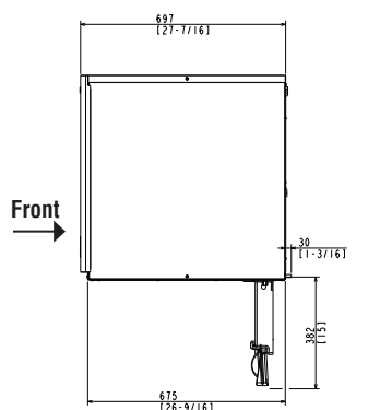
WATER-COOLED
