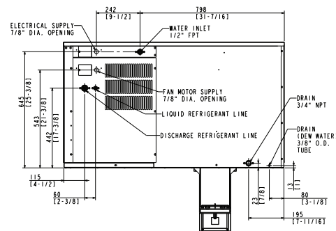
REMOTE AIR-COOLED
