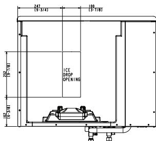
REMOTE AIR-COOLED
