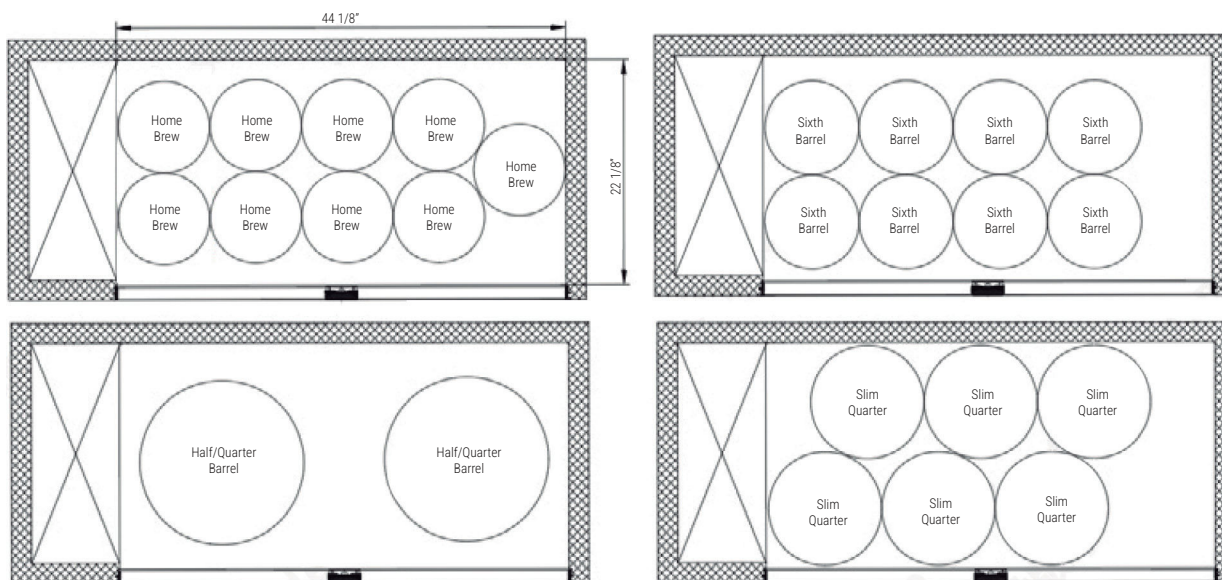
Keg configuration
