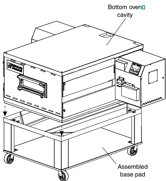
Figure 2-7. Base pad Installation
