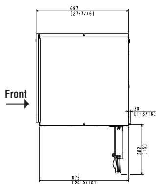
WATER-COOLED
