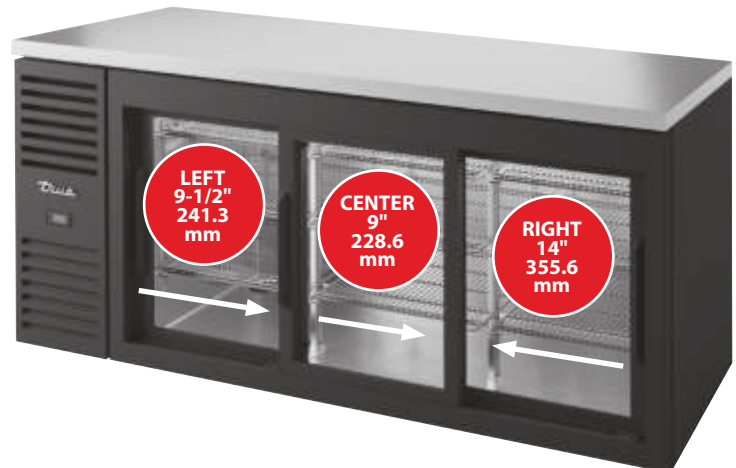
Fig. 4. Three-Door Units: Move the doors as directed to remove doors from channel.
