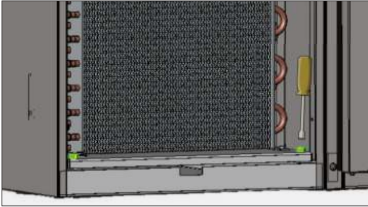
Fig. 5. Remove the condensing base bolts.
