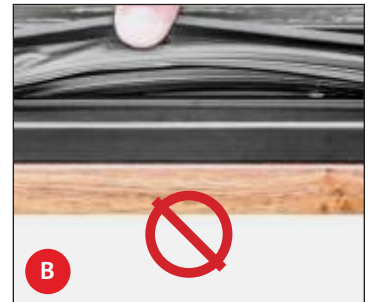
Fig. 12. Pull the side of the gasket to check its installation. A: CORRECT; gasket channel is NOT visible. B: INCORRECT; gasket channel is visible.
