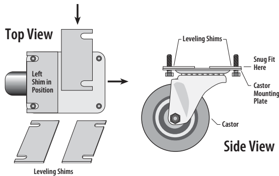
Fig. 6. Install castor shims in pairs.
