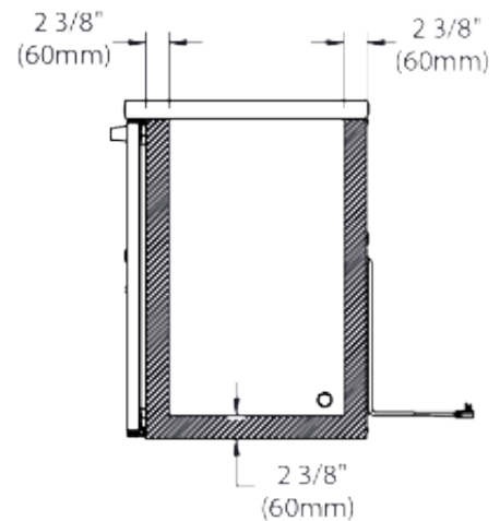
NON-CONDENSING UNIT SIDE VIEW
