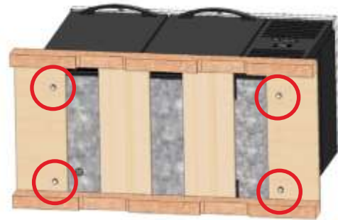
Fig. 2. Shipping bolt locations.
