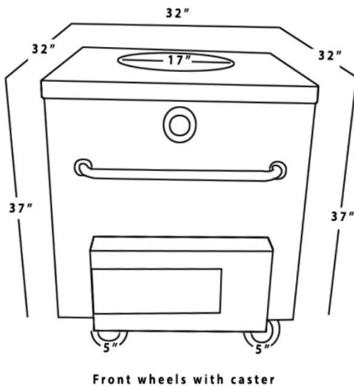
Front View of Tandoor
