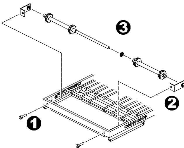
Figure 4-4. Disassembling the idler shaft
