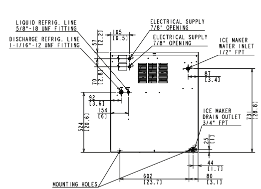
REMOTE AIR-COOLED
