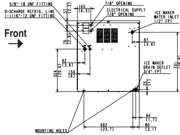
AIR-COOLED
