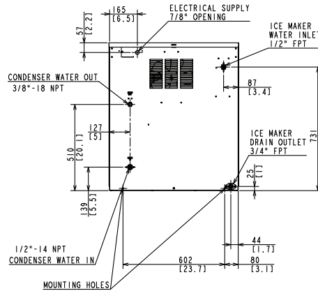
WATER-COOLED
