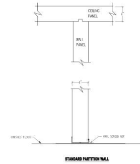
STANDARD PARTITION WALL
