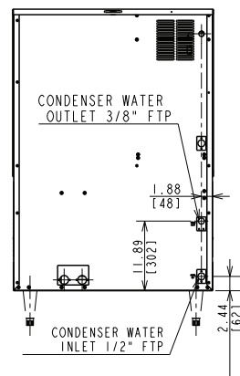
WATER-COOLED
