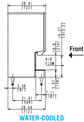
WATER-COOLED
