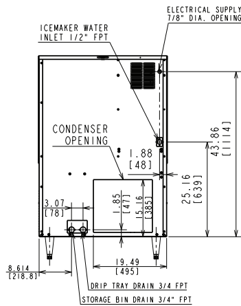
AIR-COOLED
