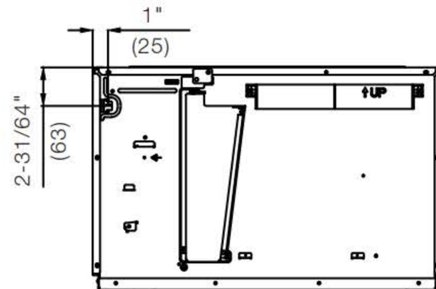
BACK VIEW
