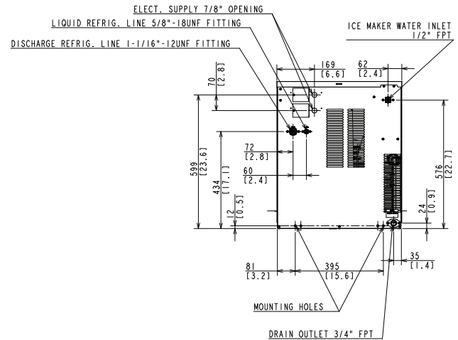
REMOTE AIR-COOLED
