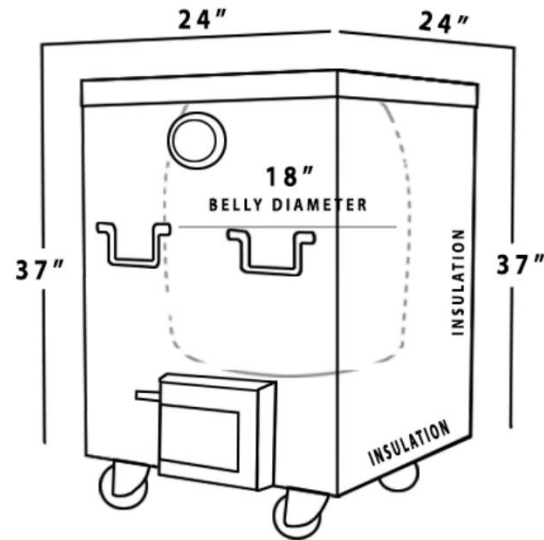
Side View of Tandoor
