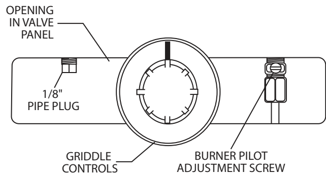
GRIDDLE PILOT VALVE
