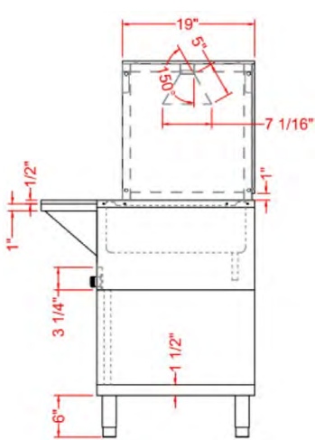
SIDE
