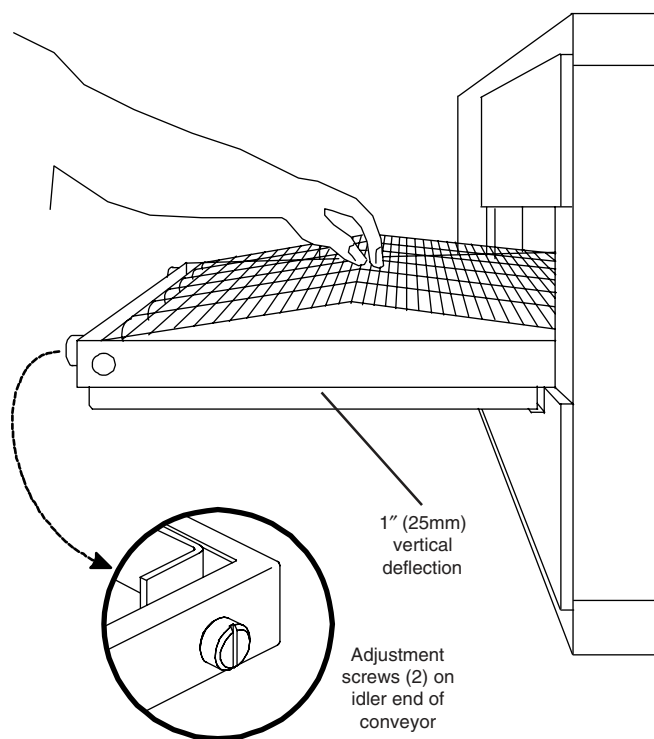
Figure 2-14. Conveyor Belt tension
