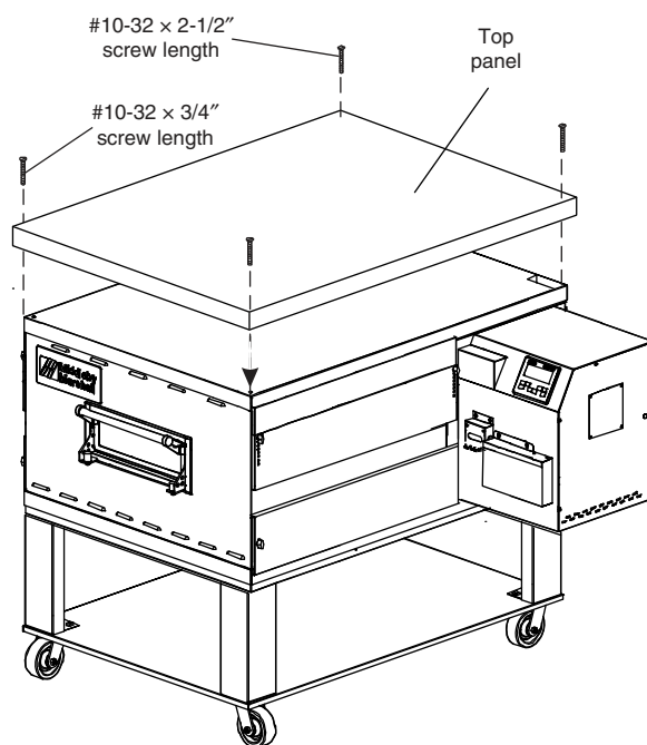
Figure 2-8. Top panel installation
