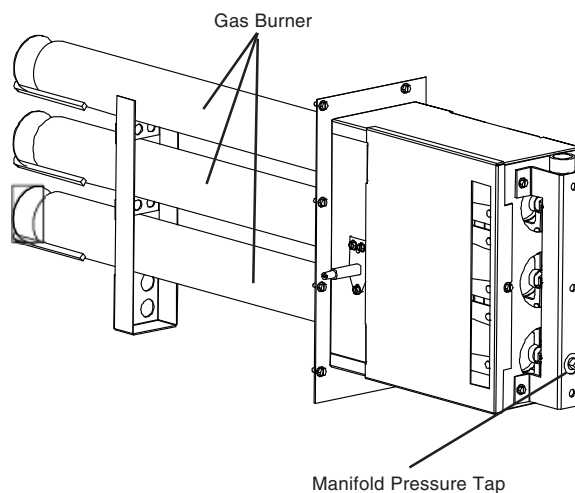
Figure 2-19. Gas Burner Assembly
