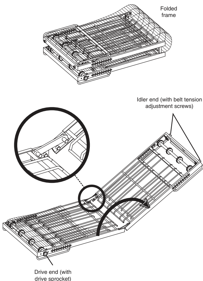
Figure 2-12. Conveyor installation
