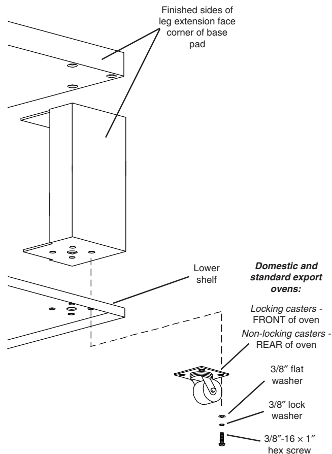
Figure 2-6. Leg extension and casters installation
