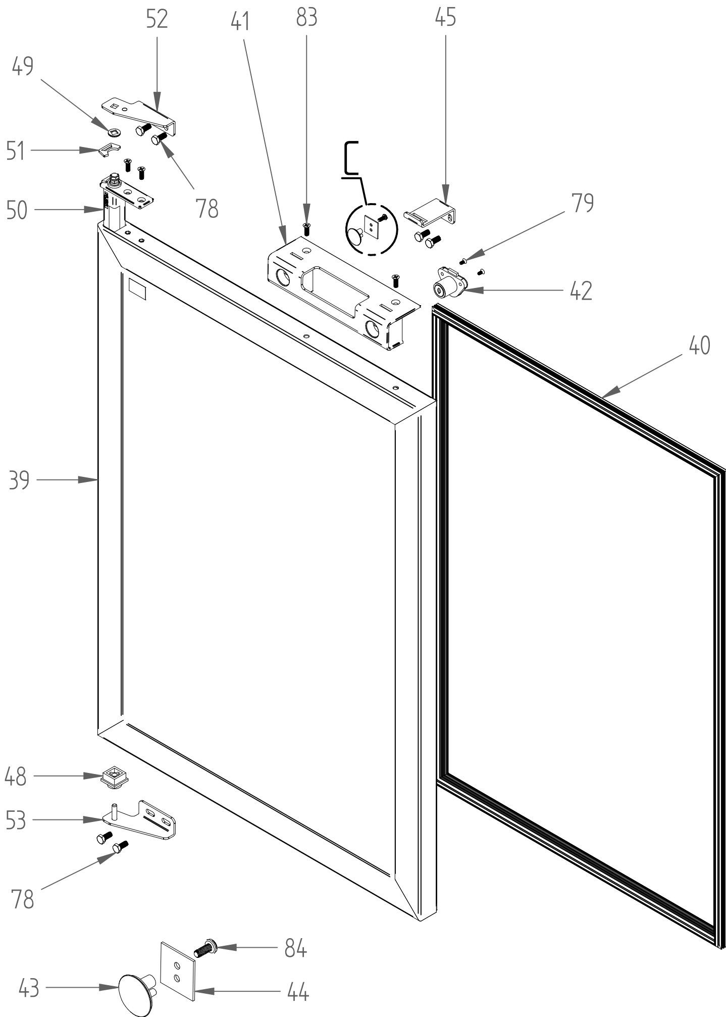
DETAIL C
