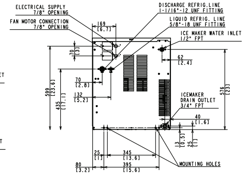
REMOTE AIR-COOLED
