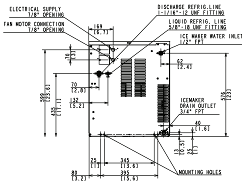
AIR-COOLED
