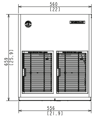
REMOTE AIR-COOLED
