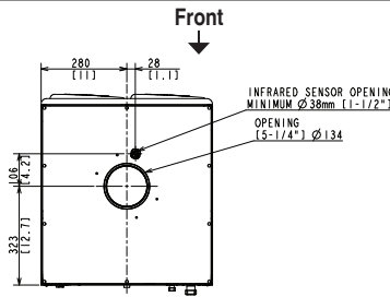
REMOTE AIR-COOLED
