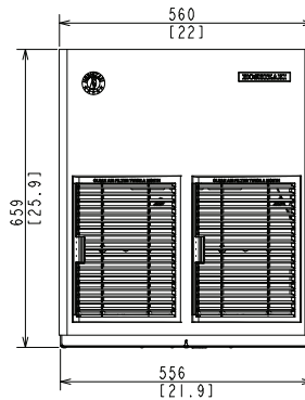
WATER-COOLED
