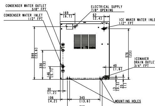
WATER-COOLED
