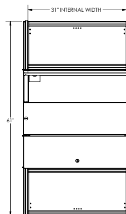
PLAN VIEW
