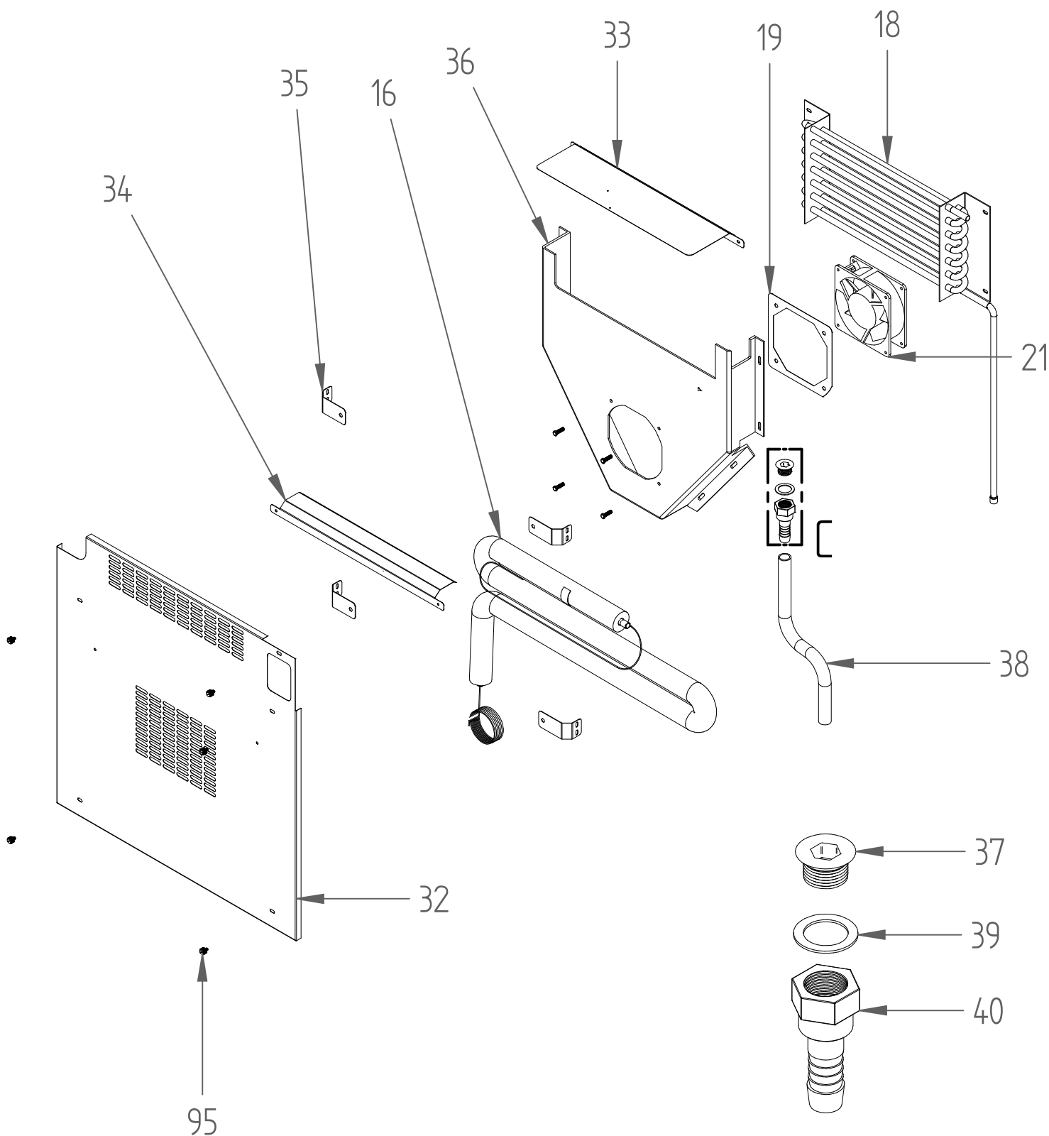
DETAIL C
